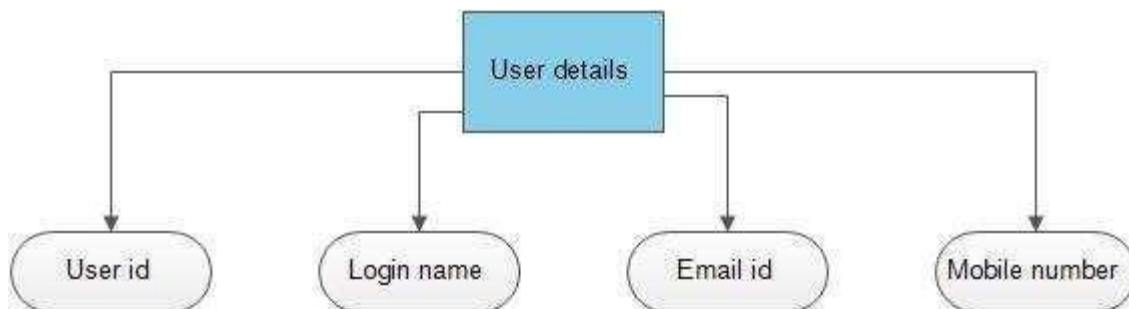
Fig 3.6: User Details
