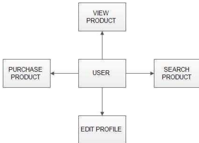
Fig 1.7: User Module
